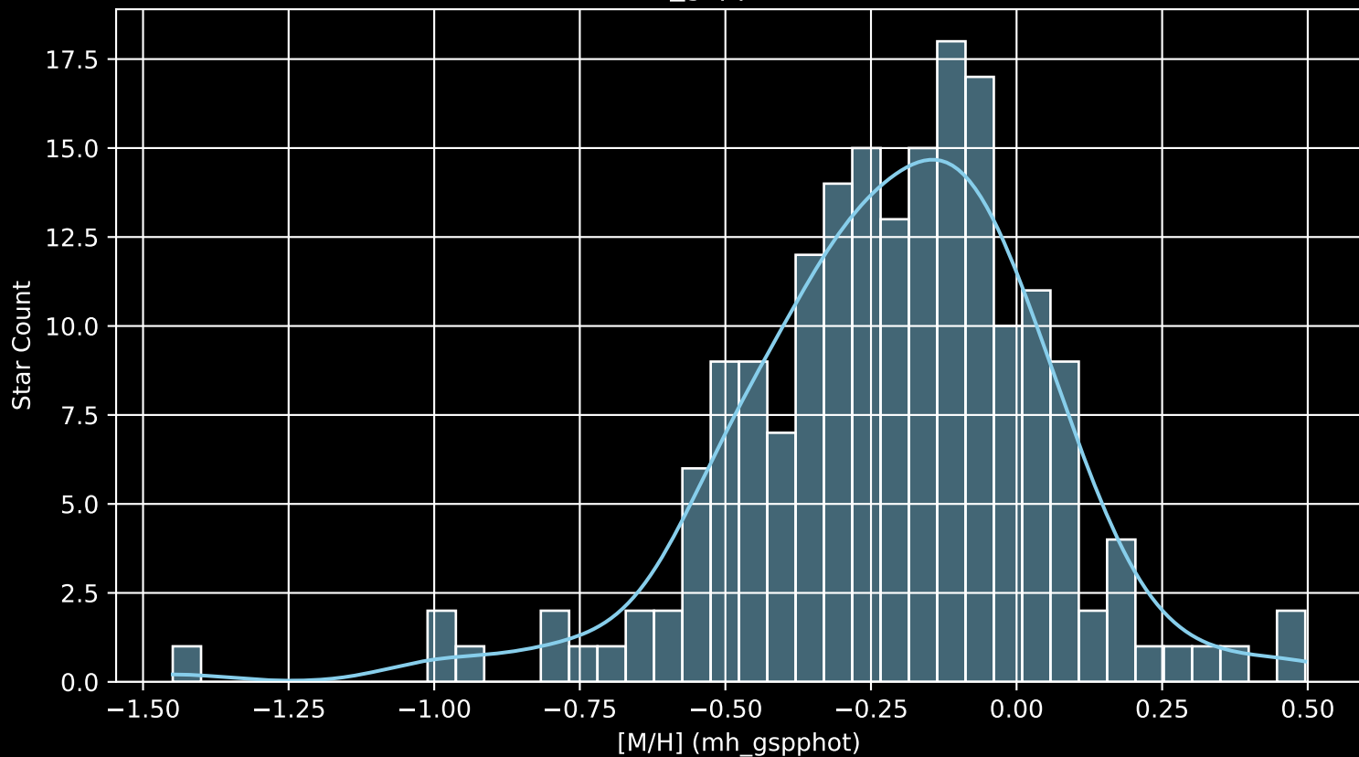
APOGEE DR17 Field: [CVZTILE_103+38_btx [M/H] (mh_gspphot) (n= 189)
