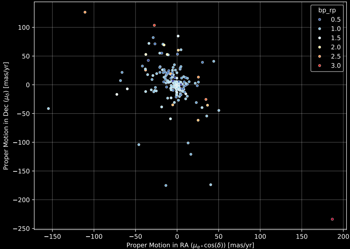
APOGEE DR17 Field: [CVZTILE_103+38_btx] Proper Motion Diagram (n= 193)
