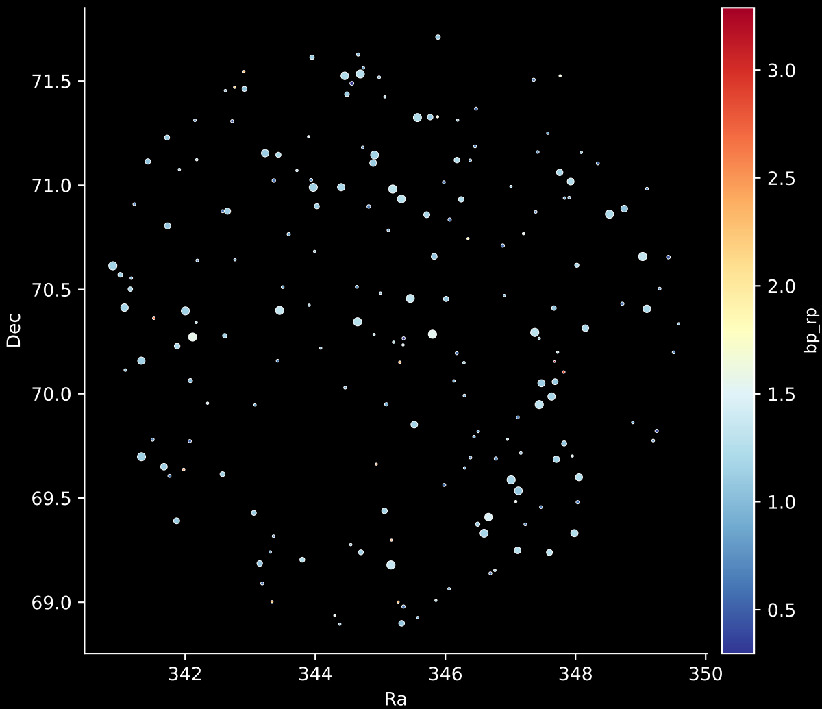
APOGEE DR17 Field: [CVZTILE_103+38_btx] Stars: 193
