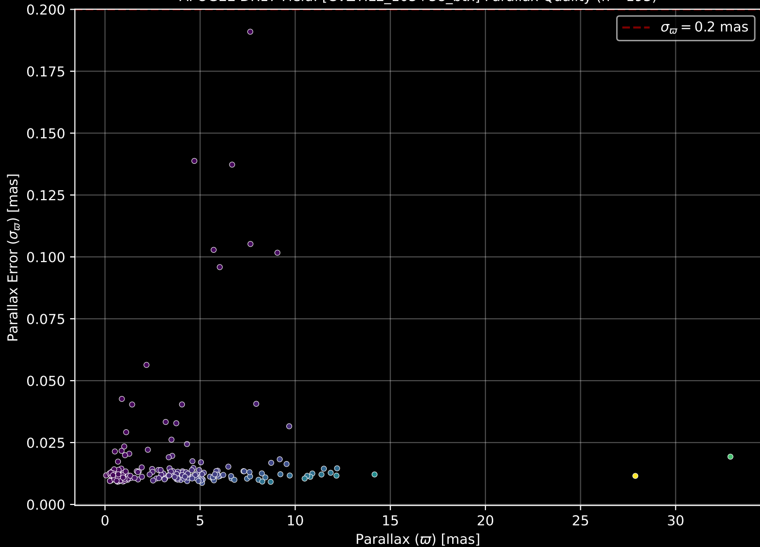
APOGEE DR17 Field: [CVZTILE_103+38_btx] Parallax Quality (n= 193)
