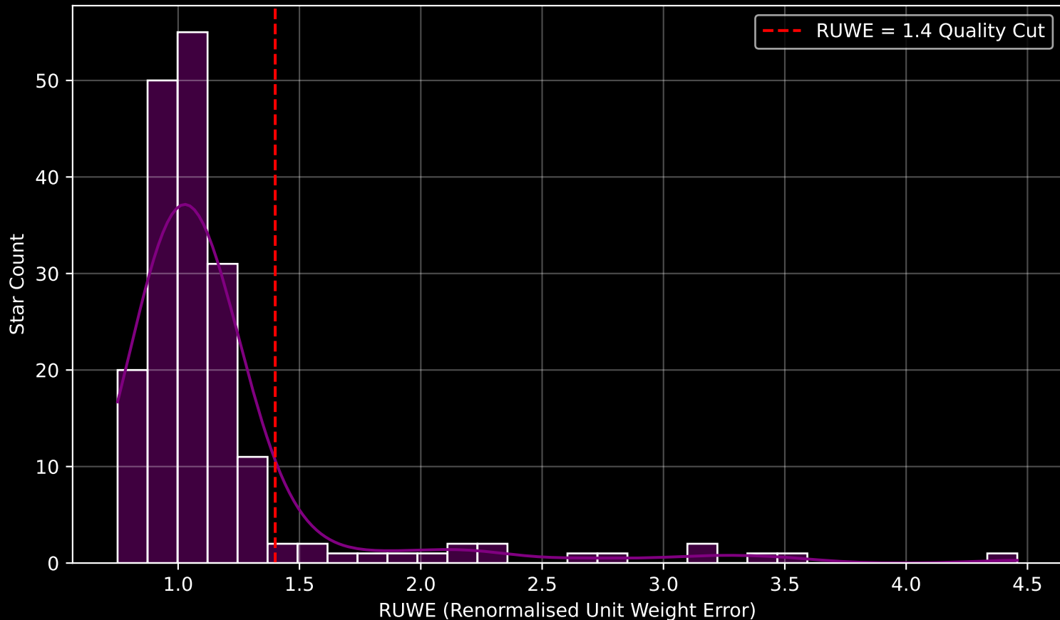
GAPOGEE DR17 Field [CVZTILE_103+38_btx] RUWE Distribution (n= 186)
