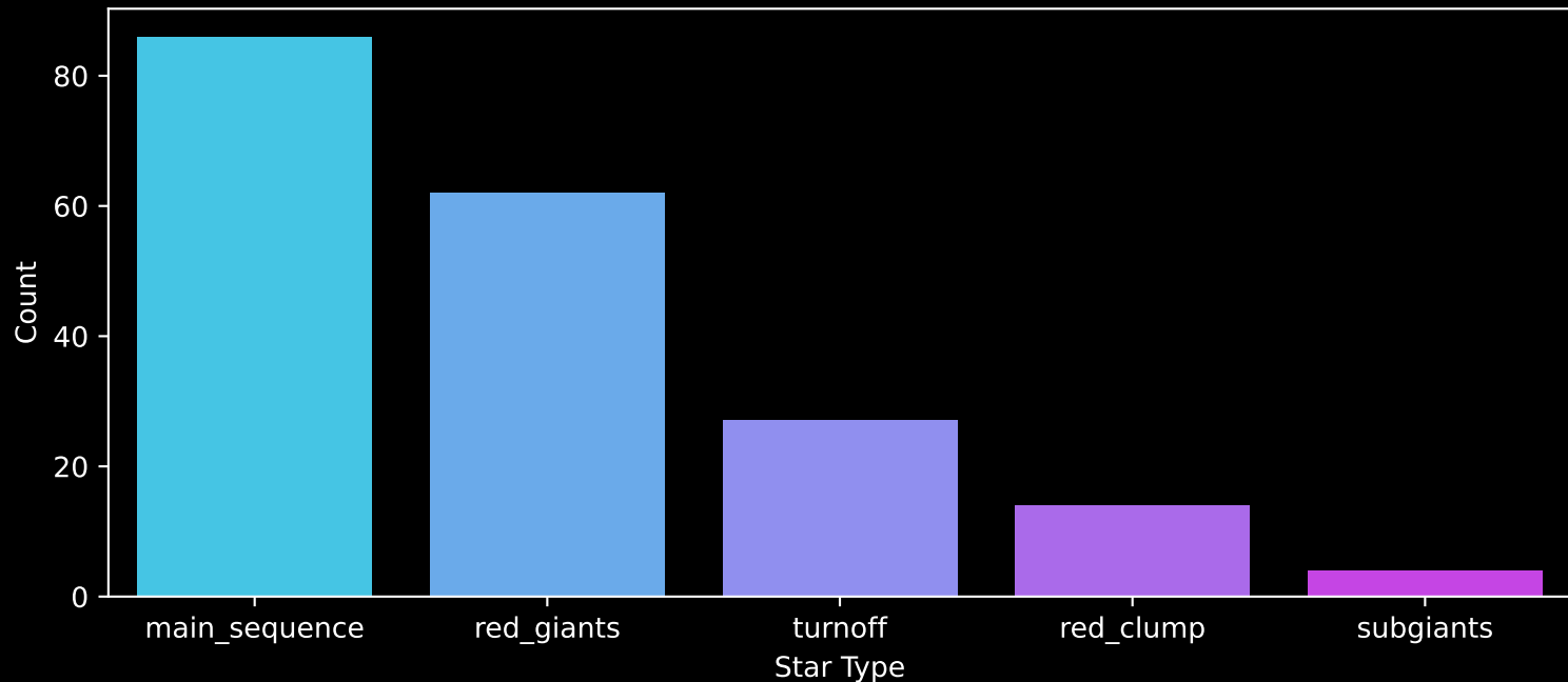
APOGEE DR17 Field: [CVZTILE_103+38_btx] Count plot of Star Type
